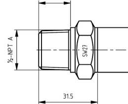
Fig. 7 - 1/2 NPT A
