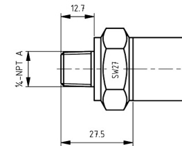
Fig. 6 - 1/4 NPT A
